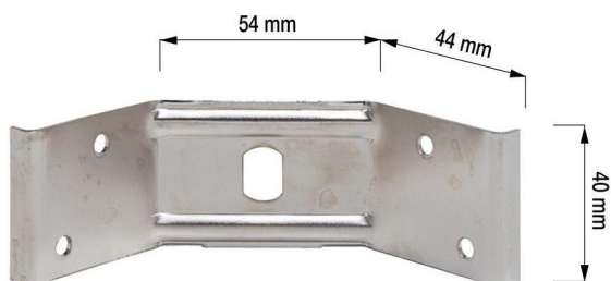
Angolare - Misure: 40/54/44 Angle bracket - Measures: 40/54/44 Winkel - Maßen: 40/54/44 Cod. 2.01.001
