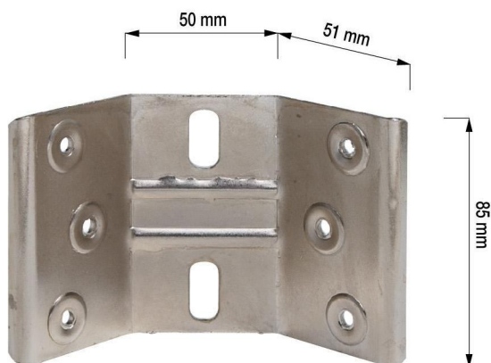
Angolare - Misure: 85/50/51 Angle bracket - Measures: 85/50/51 Winkel - Maßen: 85/50/51 Cod. 2.01.007.Z02
