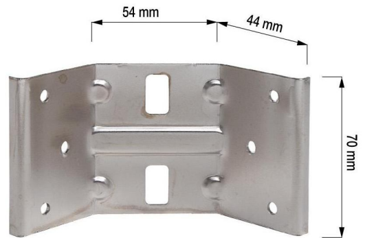
Angolare - Misure: 70/54/44 Angle bracket - Measures: 70/54/44 Winkel - Maßen: 70/54/44
