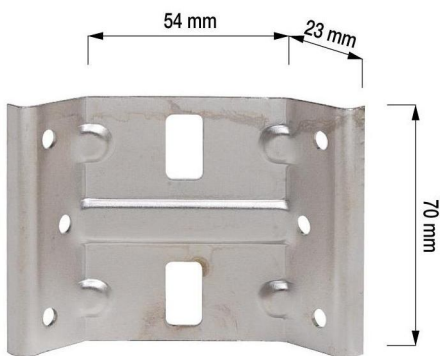
Angolare - Misure: 70/54/23 Angle bracket - Measures: 70/54/23 Winkel - Maßen: 70/54/23
