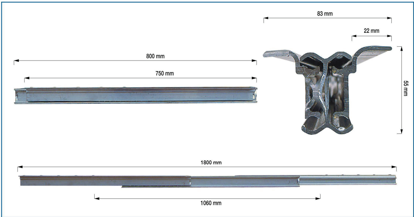
Guida telescopica in ferro o alluminio. Iron or aluminium telescopic slide. Teleskopische Eisen / Aluminiumführung.
